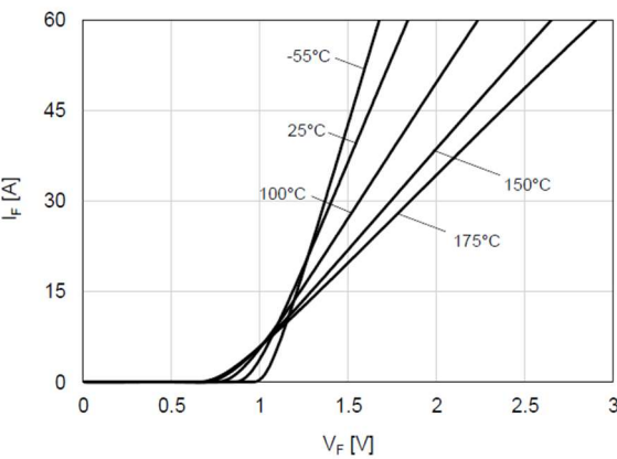
Figure 3 Forward Characteristics
