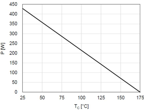
Figure 1. Power Derating
