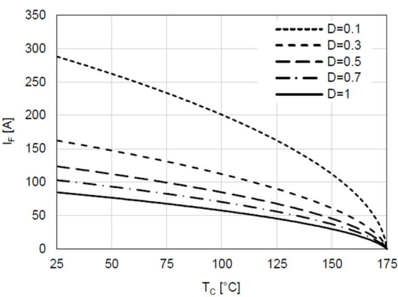
Figure 2. Current Derating
