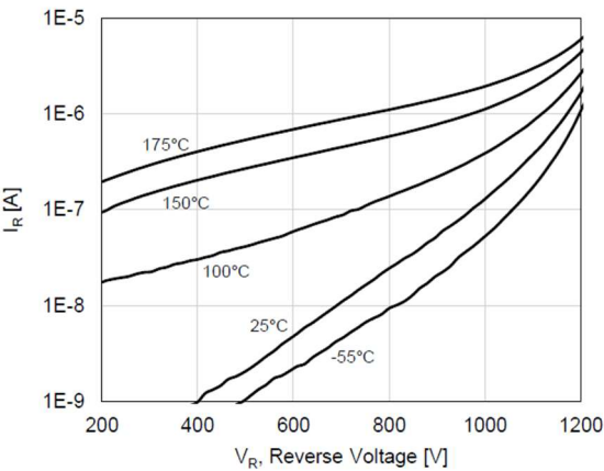
Figure 4. Reverse Characteristics
