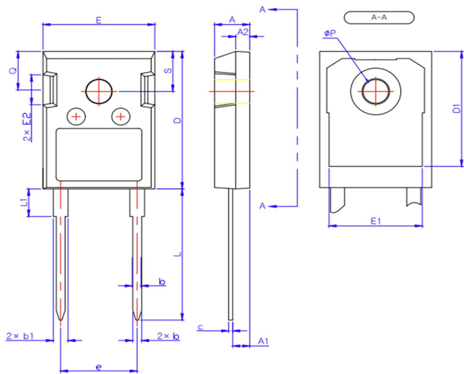
TO-247-2L
